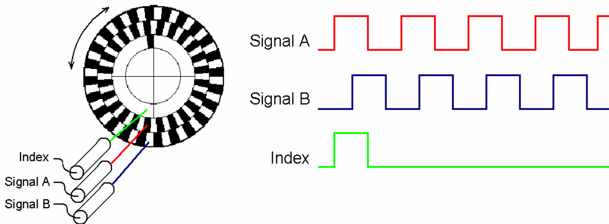
FIGURE 1. TYPICAL SIGNALS PRODUCED BY A QUADRATURE ENCODER.
