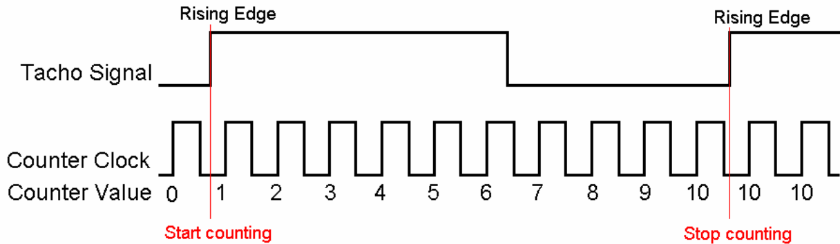
FIGURE 3. THE PRINCIPLE OF OPERATION OF THE EDGE TO EDGE MEASUREMENT.
