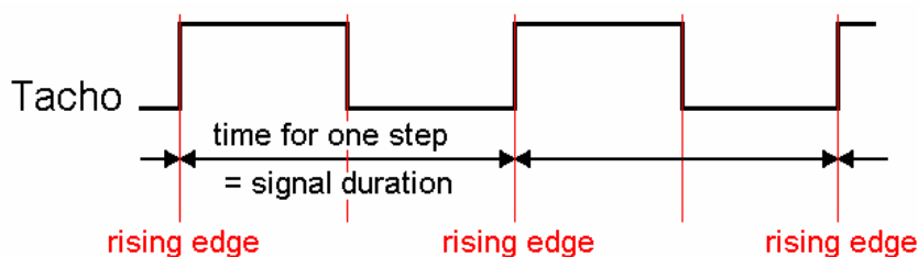
FIGURE 2. A DETAILED GRAPH OF THE TIME RELATIONS AND THE PULSE SIGNAL AND THE FUNCTION OF THE EDGE-TO-EDGE MEASUREMENT.
